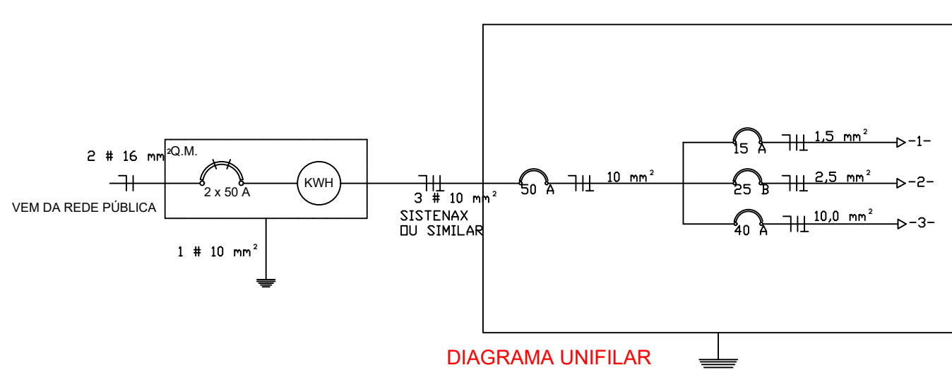
DIAGRAMA UNIFILAR
